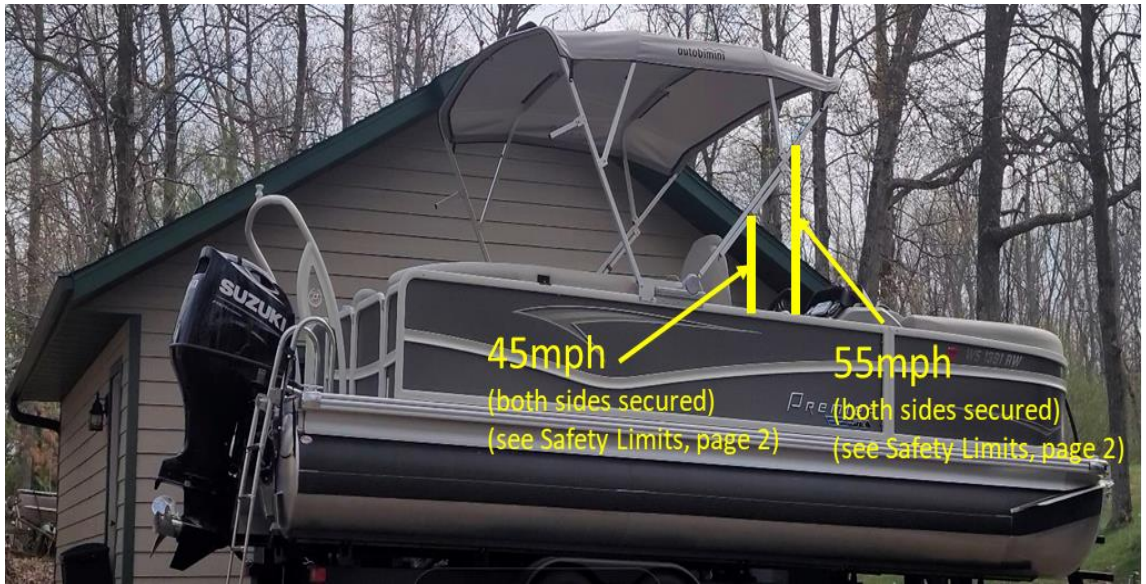
Front support arms at 1/3 (45mph) or 2/3 (55mph) speed limit locations (See Safety).
