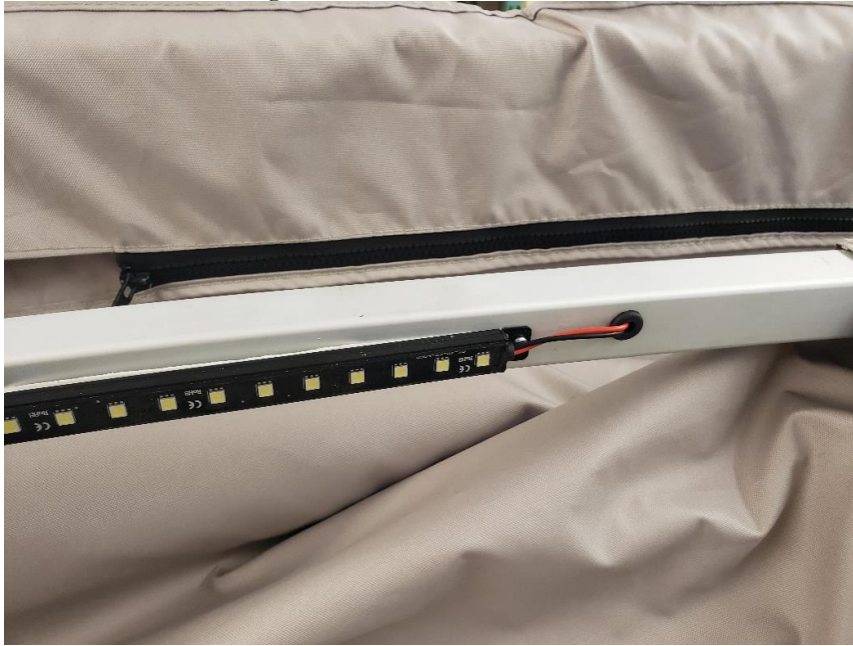
LED light wire routing in 2 nd arch
