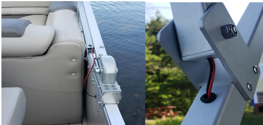
Routing of LED wire through aluminum frame
